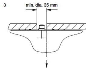
3 Pull downwards to remove radome.
